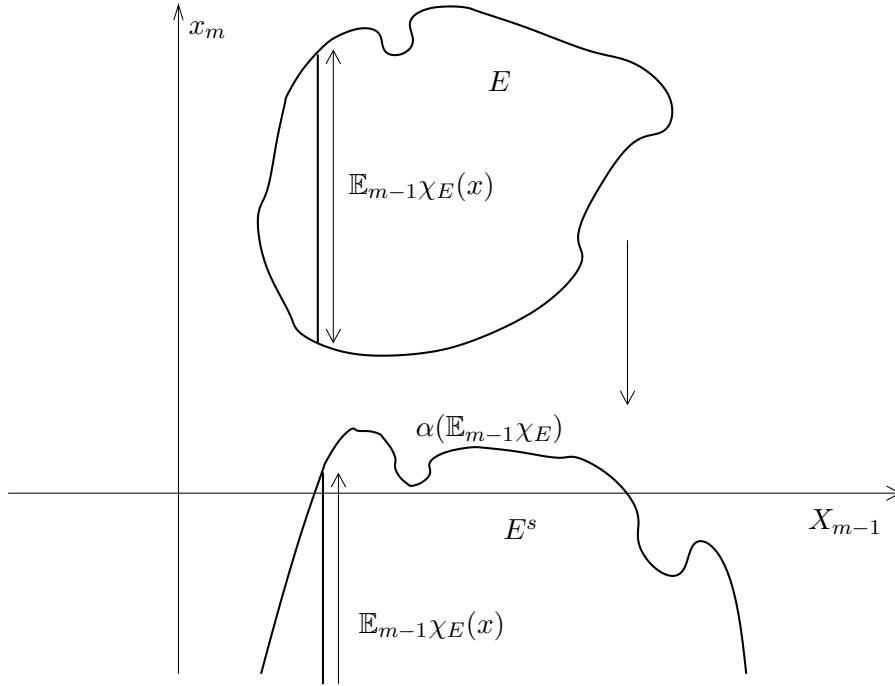
Figure 1: The Ehrhard symmetrization.
